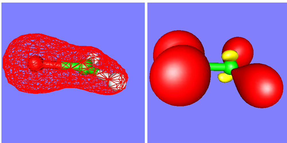
Figure 9.63: The total electron density (shown as a mesh) and the spin density (shown with solid contours) of the H 2 CO + cation radical as calculated by the RI-BP/VDZP method. Note the small negative spin density at the carbon atom. The spin density was calculated at 120x120x120 resolution which takes much longer than the DFT calculation itself.
