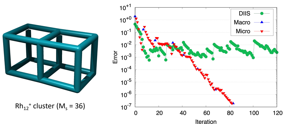
Figure 8.10: TRAHS-SCF gradient norm of a PBE/def2-TZVP calculation for a \text{Rh}_{12}^+ cluster in high-spin configuration ( M_s = 36 ). The structure was taken from Ref. 150.
